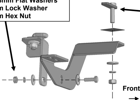
(Fig 15) Attach passenger/right Mounting Bracket to Bolt Plate and front of Support Bracket
