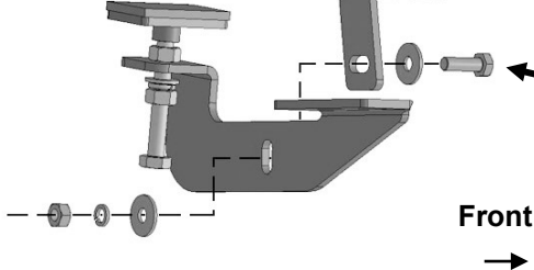
(Fig 17) Attach passenger/right center Mounting Bracket to back of Support Bracket
